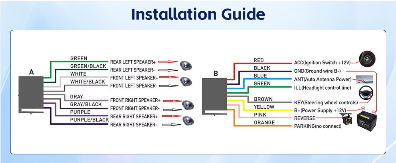
Image: Installation Guide Wiring Diagram.
