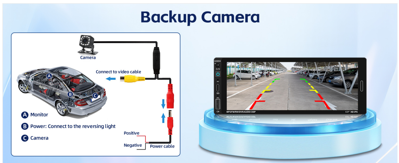
Image: Backup Camera Connection Diagram.
