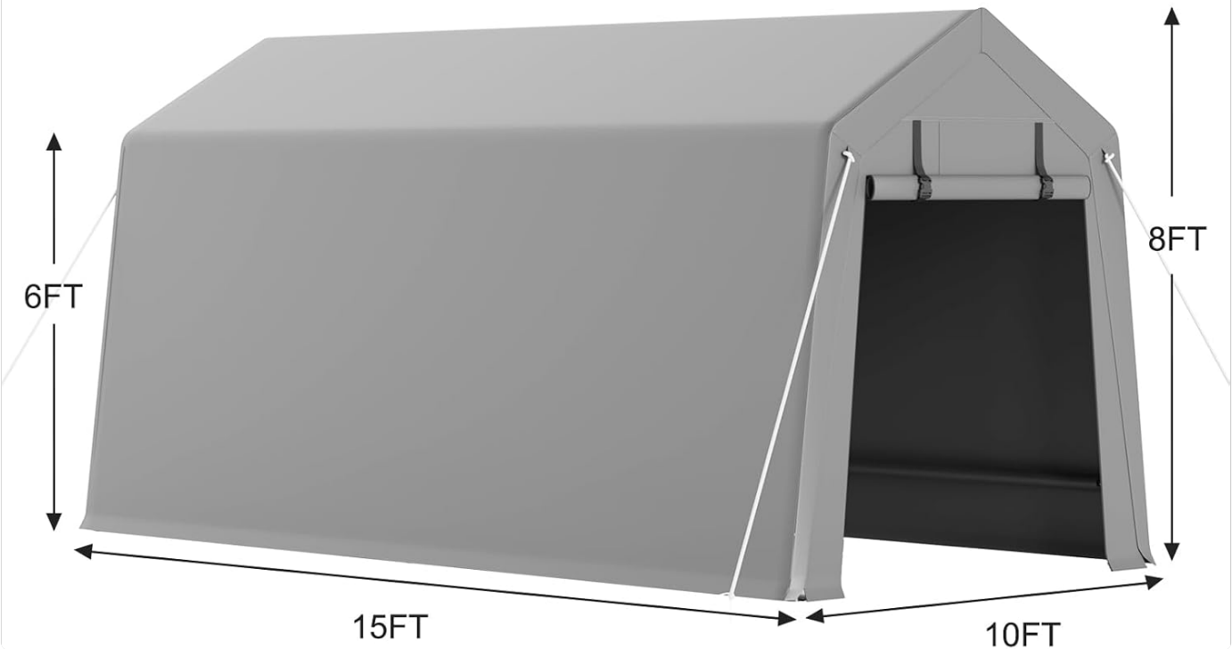
Image: Detailed dimensions of the GarveeLife 10x15 ft Carport Storage Shed.
