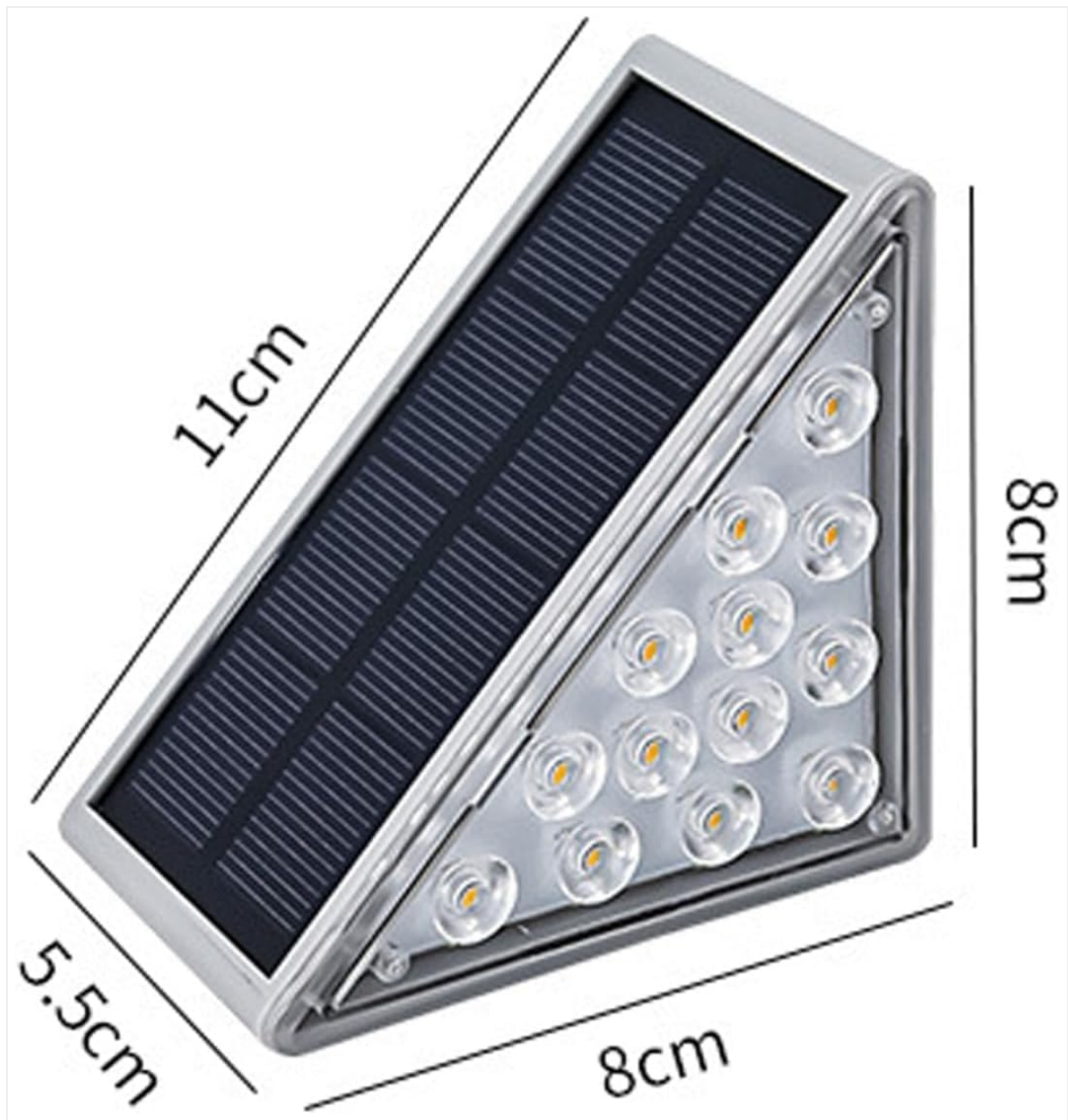
Image: A technical drawing indicating the dimensions of a single solar light unit: 11cm (top edge), 8cm (side height), and 5.5cm (depth).
