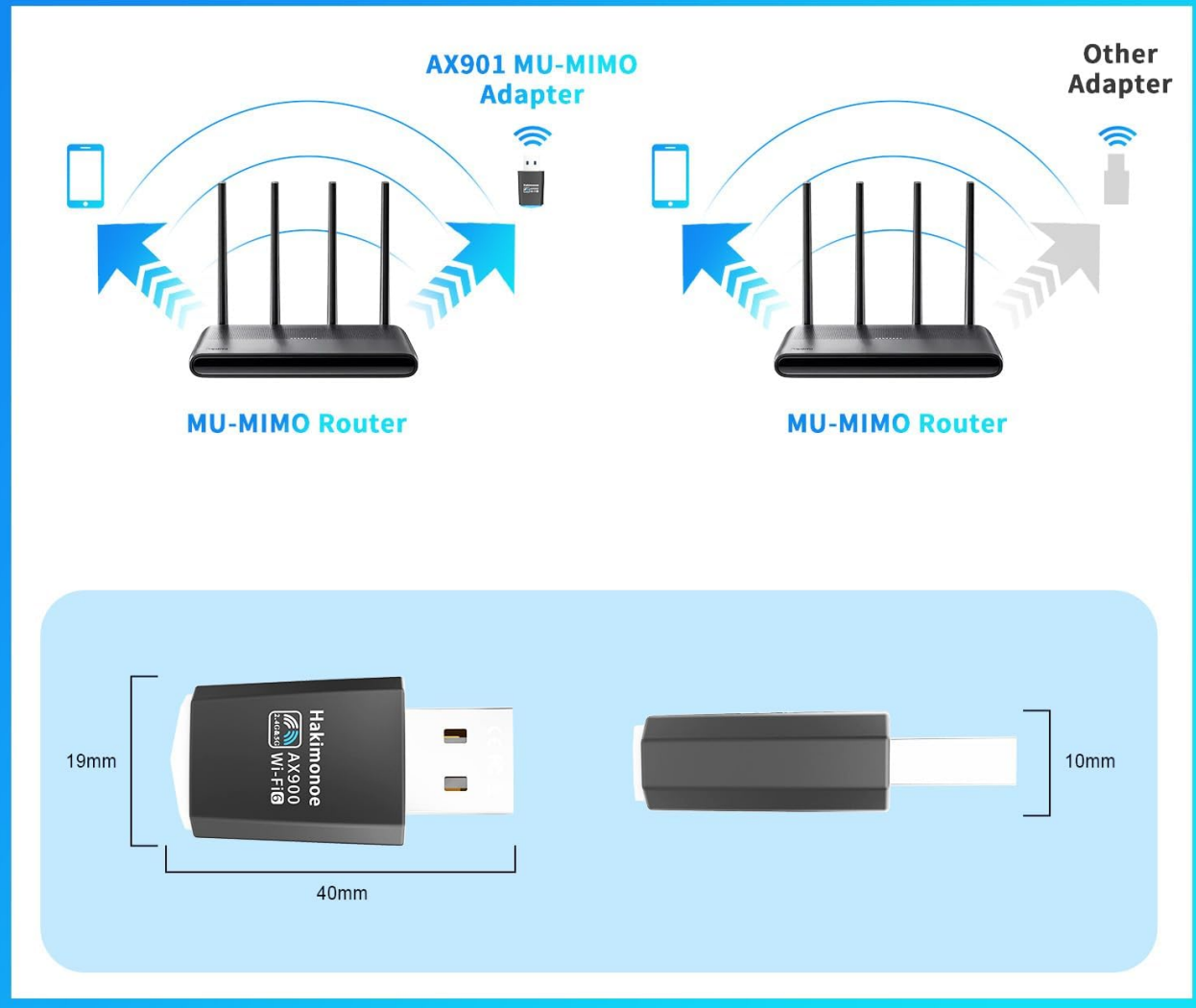
Image: A comparison diagram showing how MU-MIMO technology with the AX901 adapter improves data transmission efficiency compared to traditional adapters, allowing multiple devices to receive data simultaneously.
