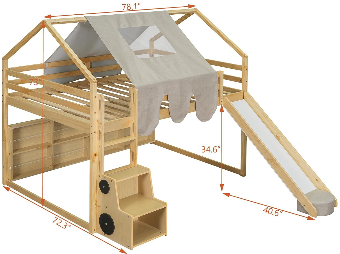
Figure 4.2.1: Overall dimensions of the loft bed, including height, length, and width of the bed, slide, and stairs.
