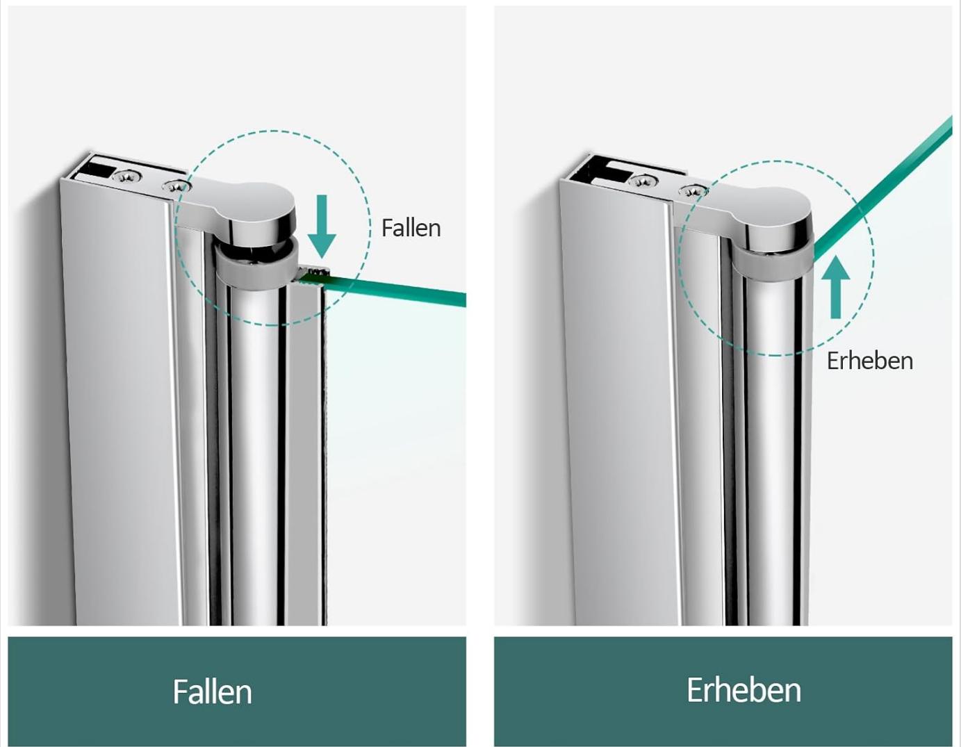
Figure 5: The integrated 4mm lift and lower mechanism protects the bottom seal during movement and ensures a secure, quiet closure against the bathtub.
