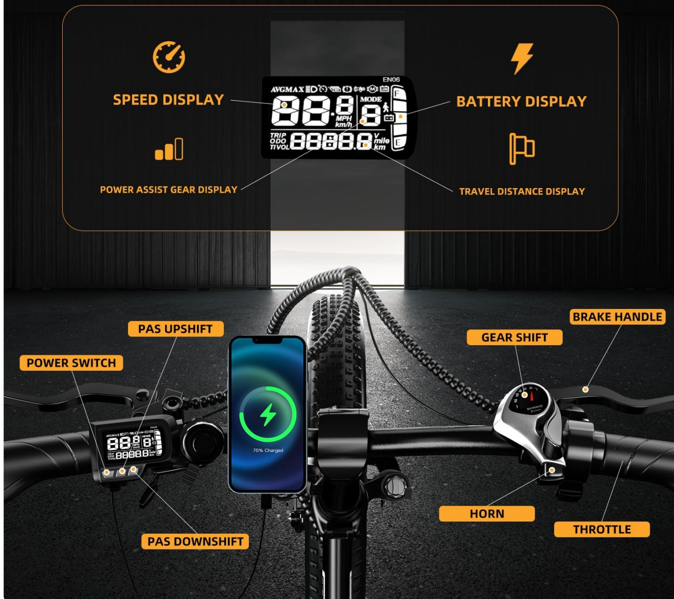
Figure 3: Close-up of the intelligent LCD display, showing speed, battery, PAS gear, and travel distance indicators.
