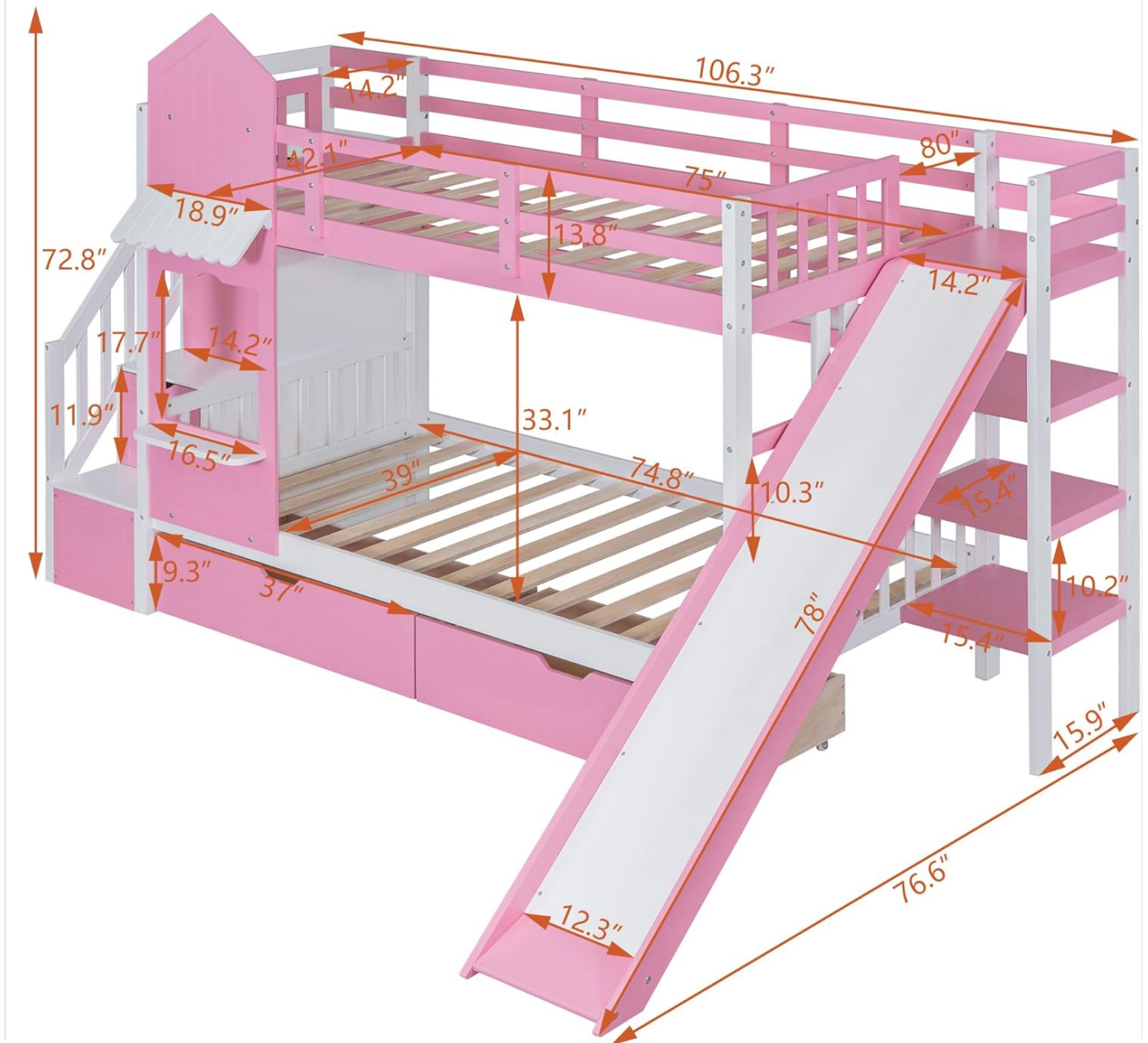
Figure 2: Detailed dimensions of the bunk bed for planning room layout and mattress selection.
