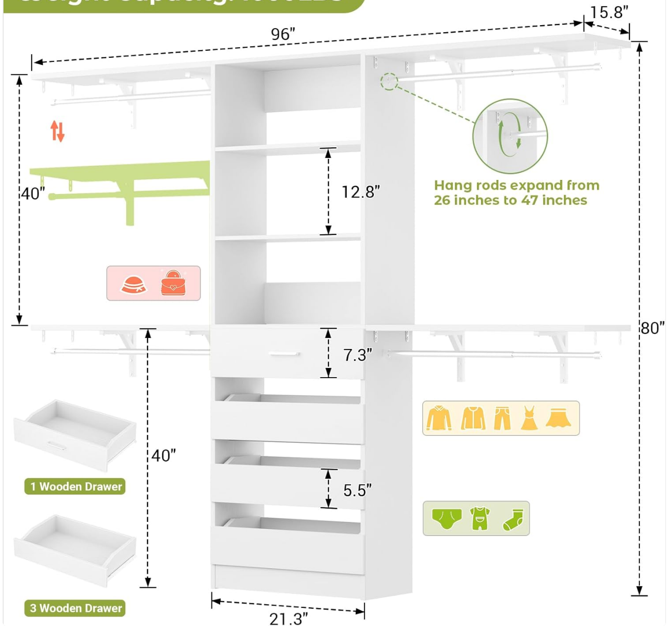
Image 8.1: Dimensional drawing of the Aheaplus Closet System, including key measurements and overall weight capacity.
