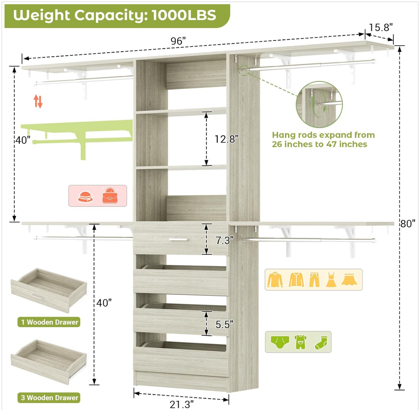
Image: Technical diagram illustrating the dimensions and weight capacity of the closet system, including the central tower, hanging rods, and drawers.
