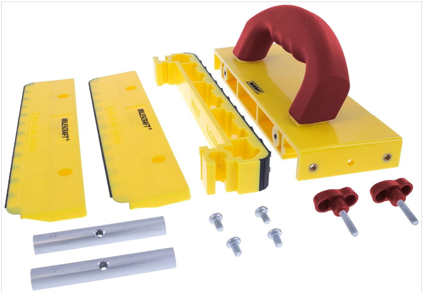
Image: All components of the Milescraft 3407 GrabberPRO LITE, including the main body, handle, two legs, and fasteners, laid out on a surface.
