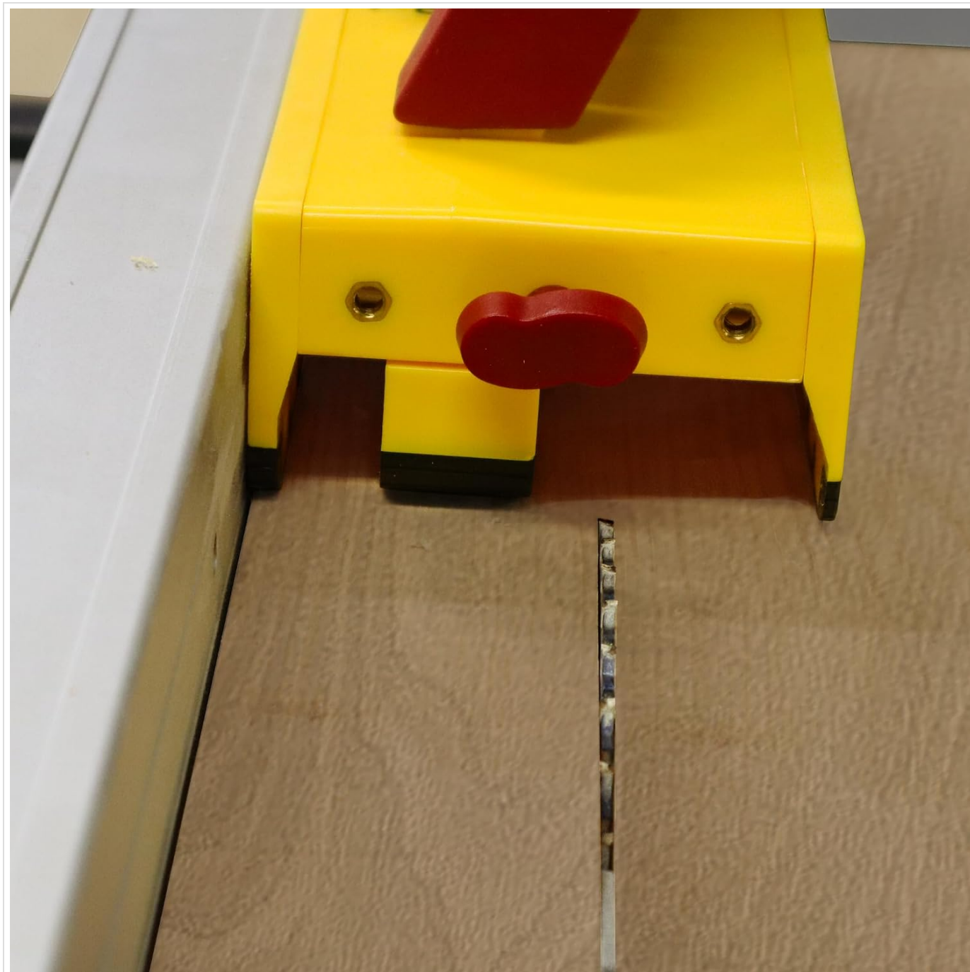
Image: A close-up view of the Milescraft GrabberPRO LITE positioned on a table saw, with its legs safely clearing the saw blade.
