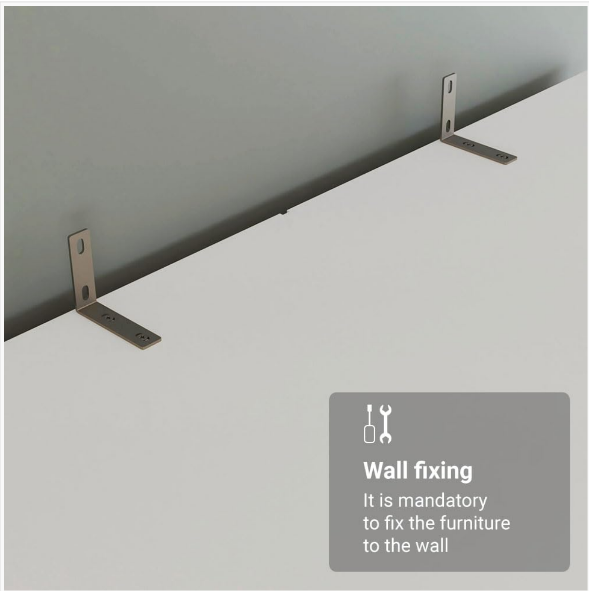
Image 2: Wall-mounting hardware for securing the cabinet.
