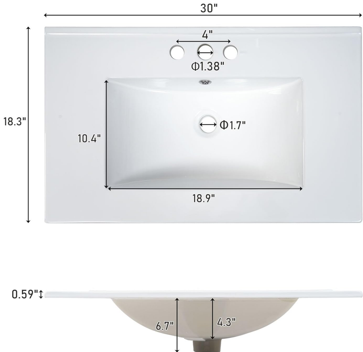
Figure 3: Detailed dimensions of the ceramic sink, showing basin measurements and pre-drilled faucet holes.
