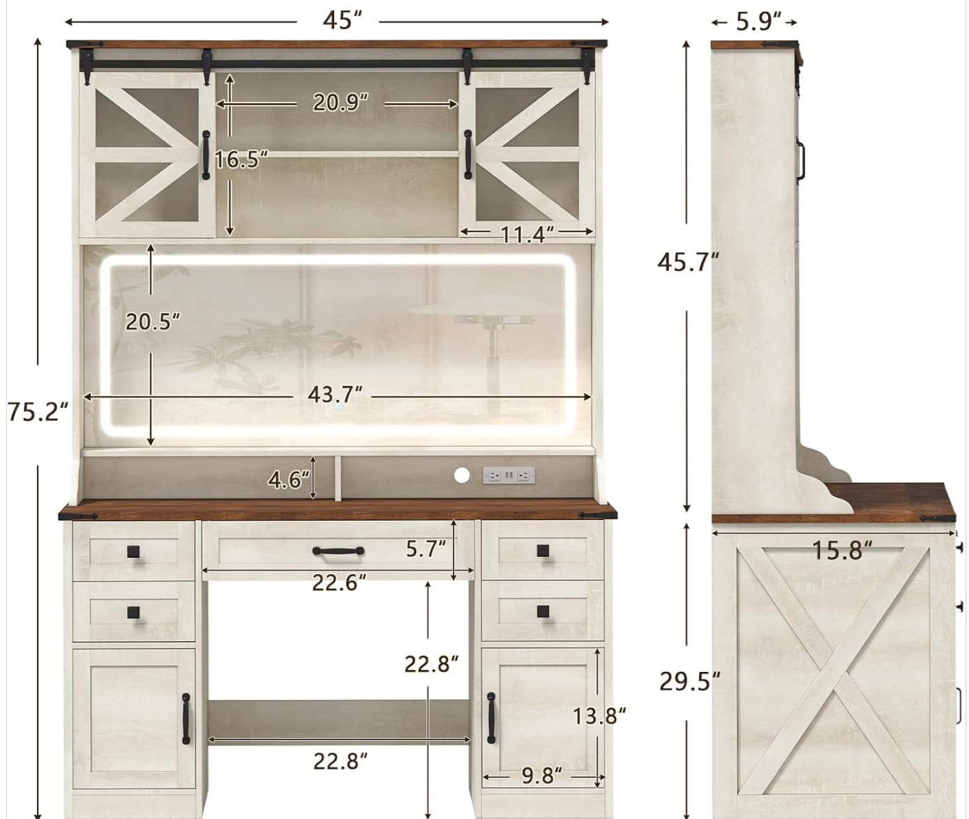
Figure 2: Detailed dimensions of the vanity desk components.
