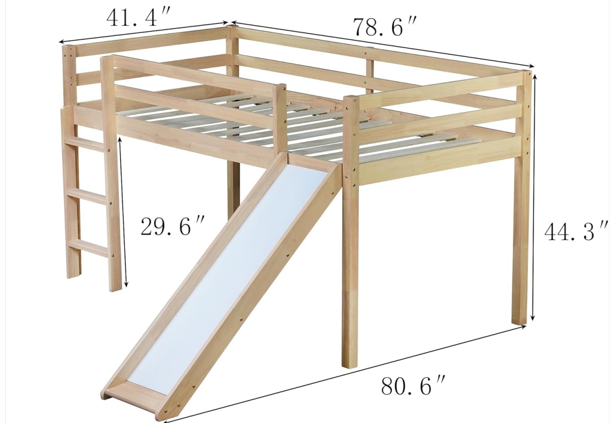
Figure 7.1: Product dimensions (L: 80.6", W: 43.4", H: 44.3").
