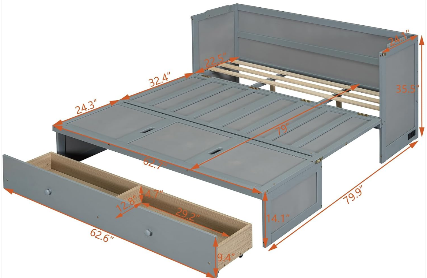
Image: Unfolded dimensions of the Murphy bed, illustrating length, width, and height of the bed frame and the integrated drawer.
