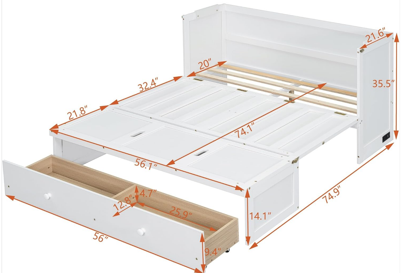
Figure 3.1: Detailed dimensions of the Murphy Bed Cabinet when fully extended as a bed. This image provides measurements for length, width, and height, including the headboard and the pull-out drawer.
