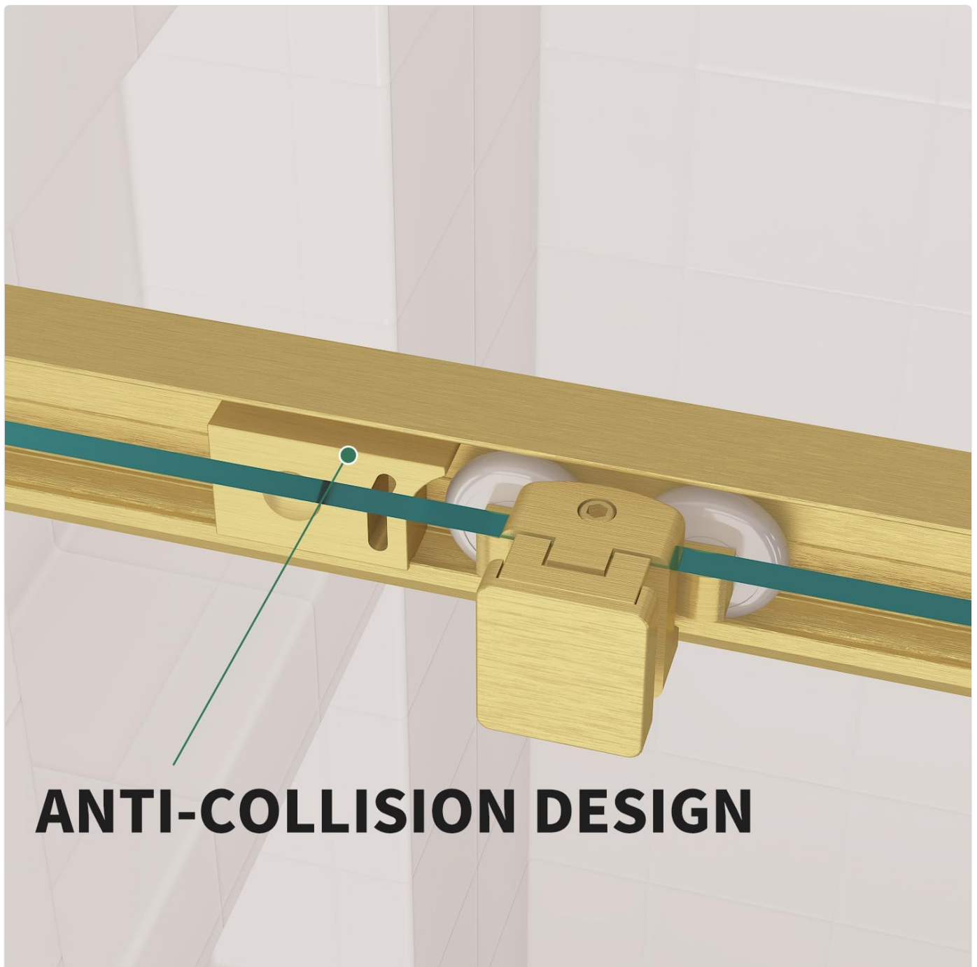
Figure 6: Adjustable size feature allowing for minor adjustments to fit varying wall conditions, and the anti-collision design for enhanced safety.
