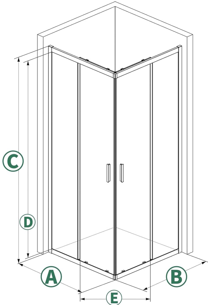
Figure 1: Overall dimensions and measurement points (A, B, C, D, E) for the shower enclosure. Ensure your space matches these specifications for proper fit.
