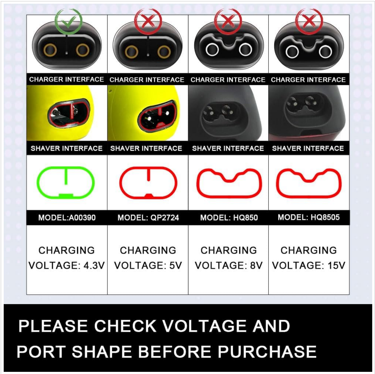
Figure 7.1: Visual comparison of charger interfaces and voltages, indicating incompatible models.
