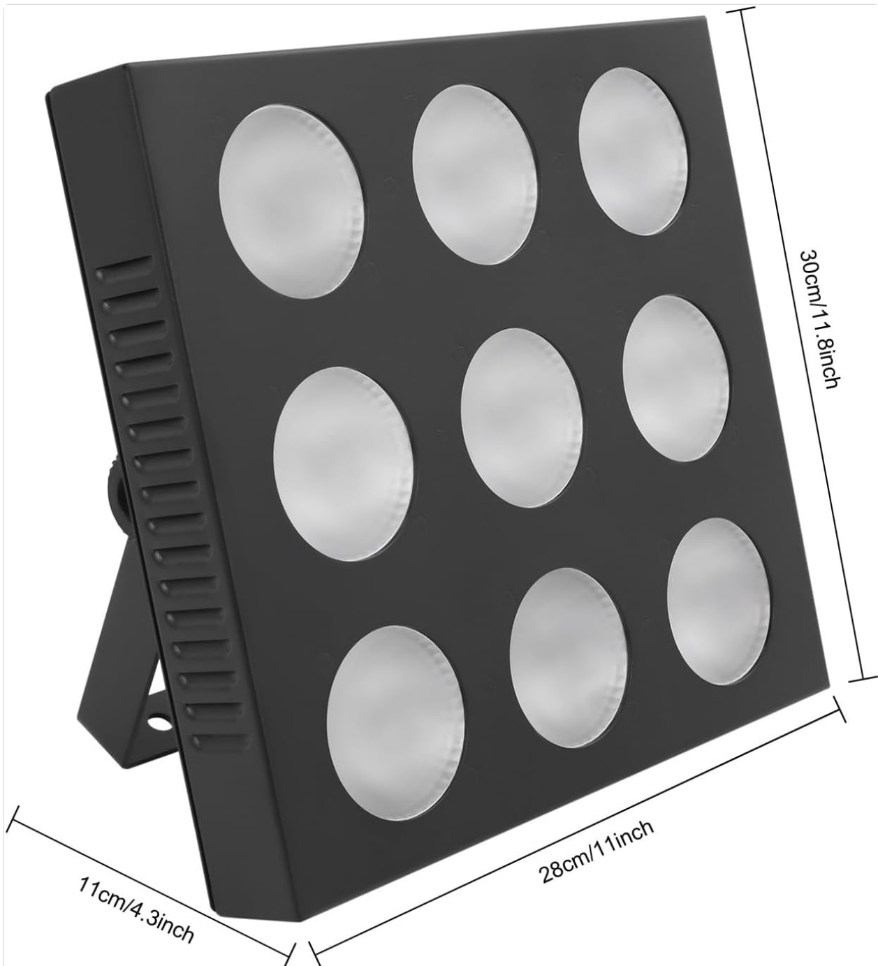
Image: The Kreiaoer Stage Light with its dimensions labeled: 30cm (11.8 inches) height, 28cm (11 inches) width, and 11cm (4.3 inches) depth. This provides a visual reference for planning installation space.
