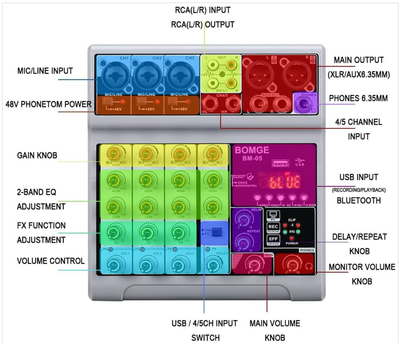
Figure 2: Detailed panel description of the BOMGE BM-05, highlighting various inputs, outputs, and controls.
