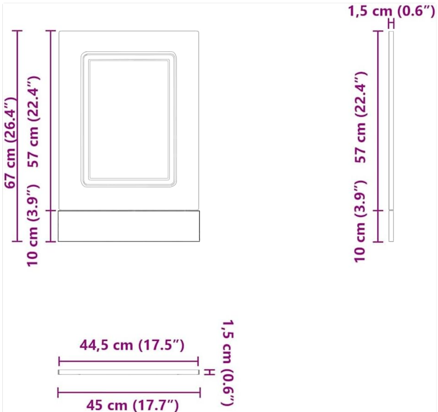
Figure 3: Detailed dimensions of the dishwasher panel for compatibility verification.
