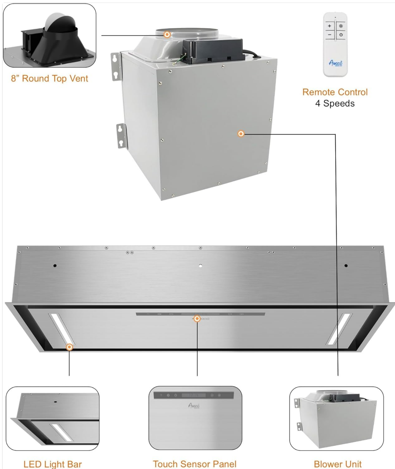
Figure 3: Components of the Awoco Flush Ceiling Mount Split Insert Range Hood, including the blower unit, 8-inch round top vent, remote control, LED light bar, and touch sensor panel.
