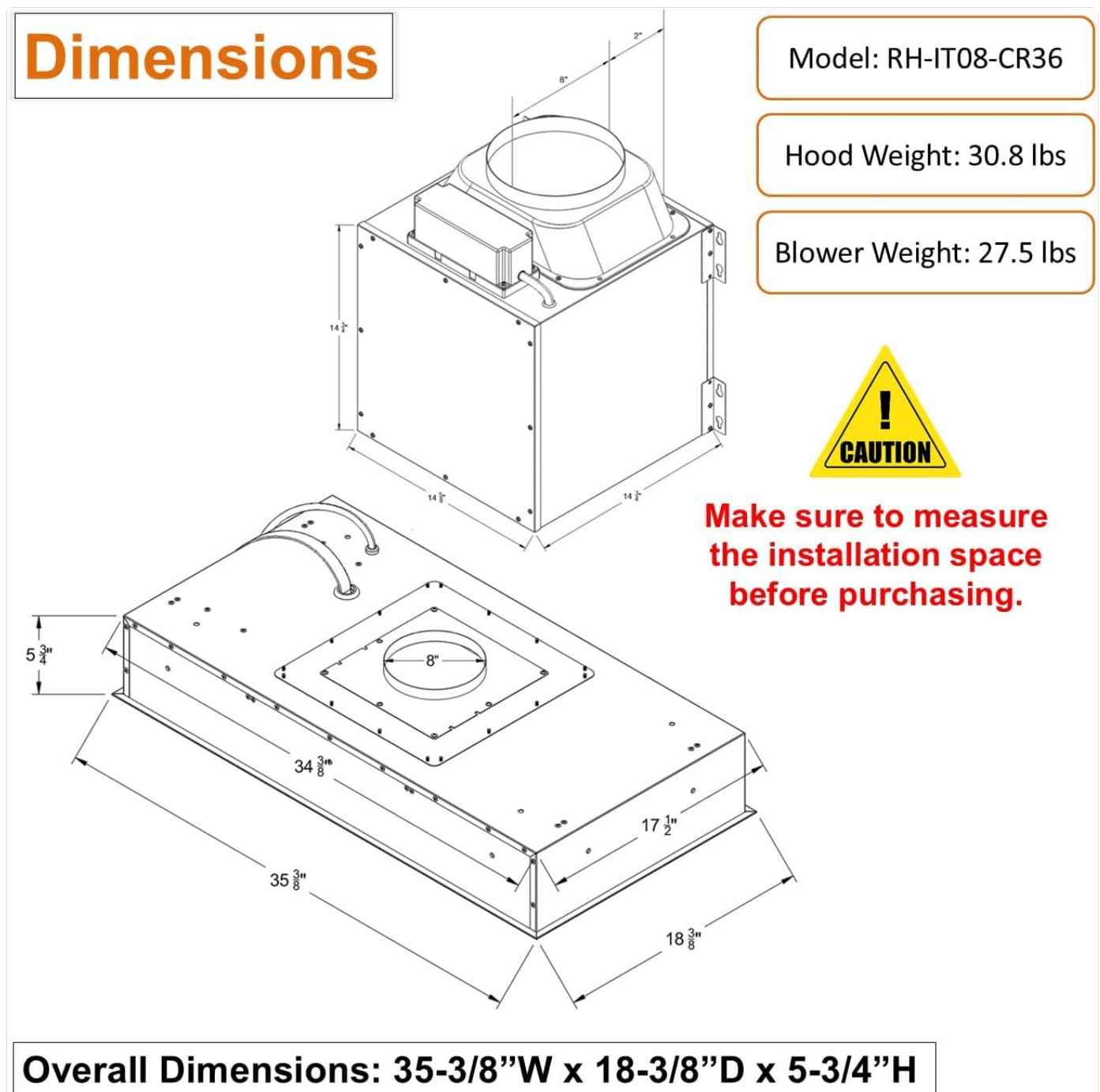
Figure 1: Overall dimensions of the hood and blower units. Model: RH-IT08-CR36. Hood Weight: 30.8 lbs. Blower Weight: 27.5 lbs.
