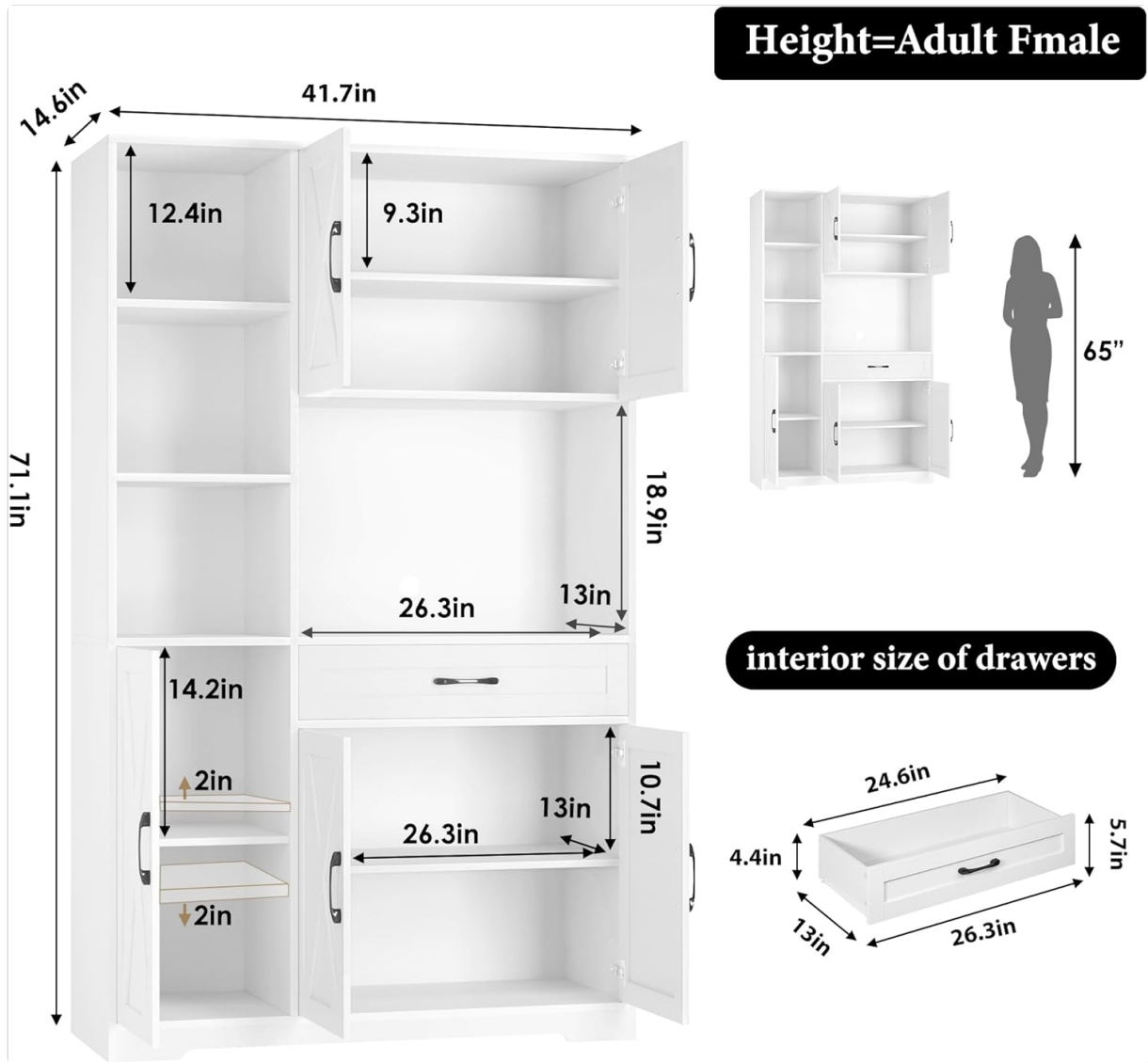
Figure 2: Detailed dimensions of the cabinet, including shelf heights and drawer interior size. The overall dimensions are 14.6"D x 41.73"W x 71"H.
