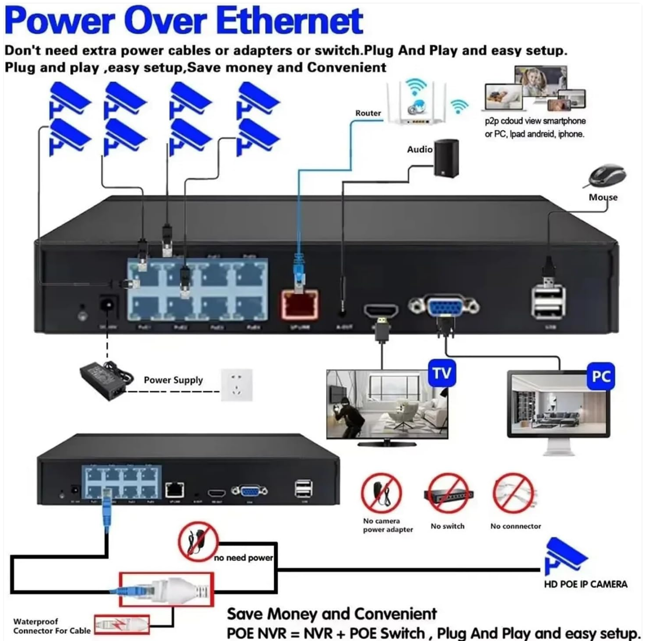
Figure 4.1: POE NVR System Connection Diagram. Connect cameras to NVR POE ports, NVR to router, and NVR to a monitor and mouse.
