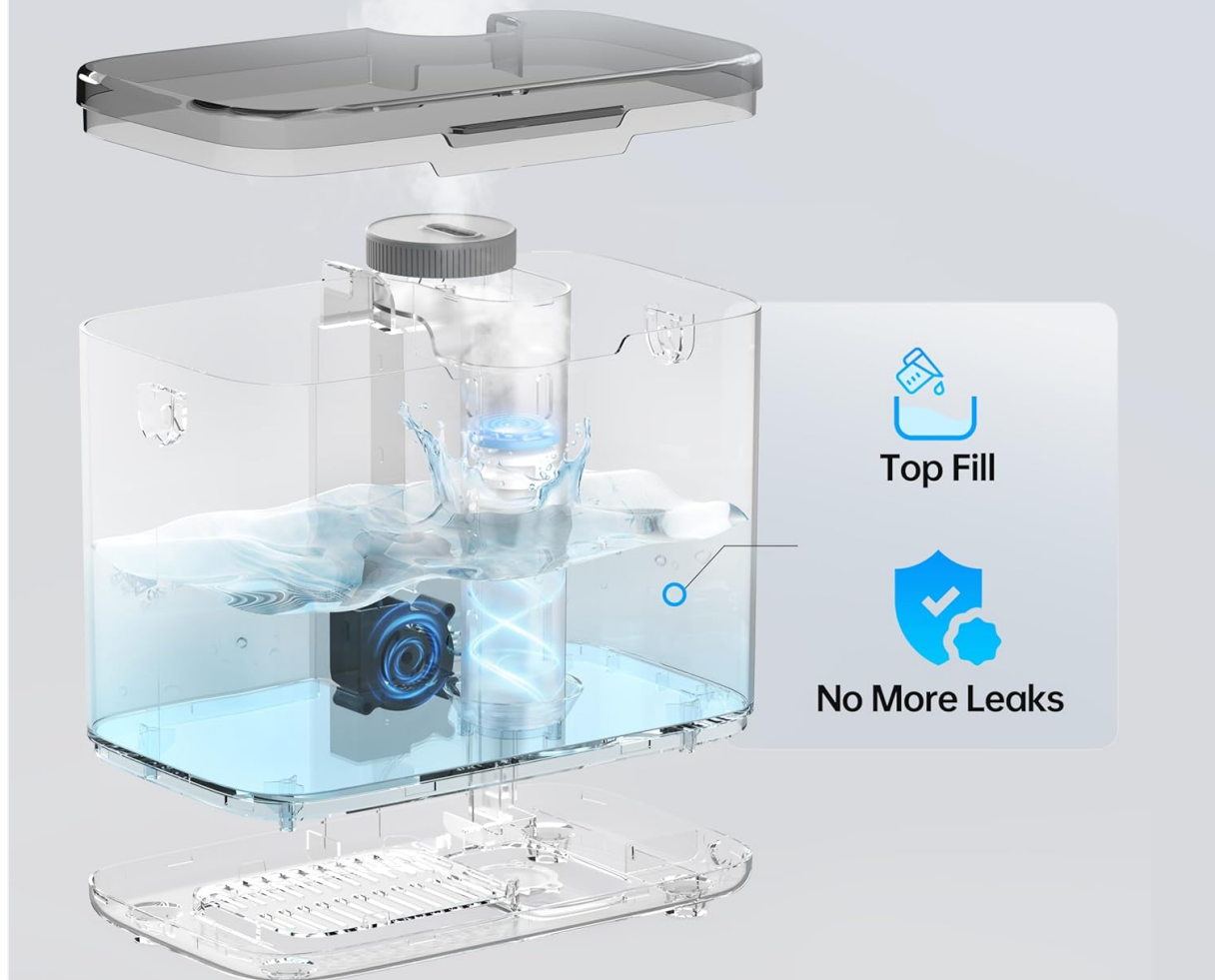
Figure 2.2: Internal view of the Luri UM-HHM001 humidifier showing the advanced integrated water tank and top-fill design.
