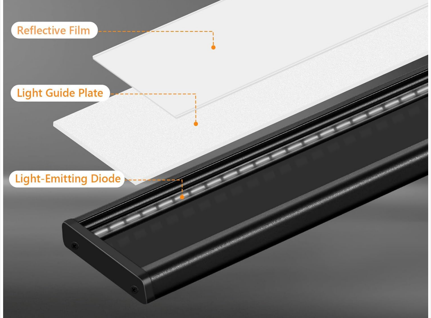
Figure 2.3: Side-Emitting Light Design for even light distribution.
