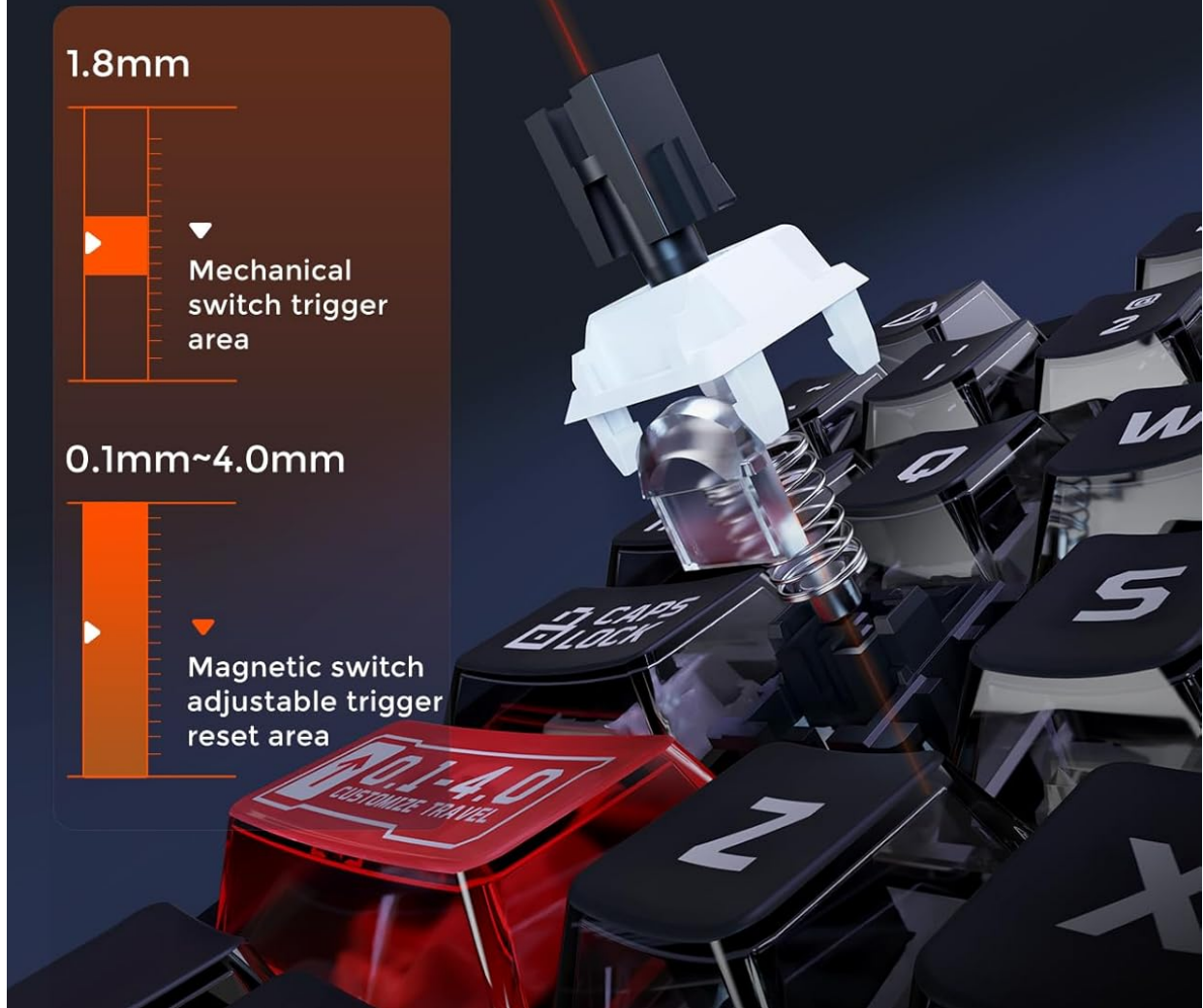
Figure 6: Rapid Trigger Mode functionality of the EK75RT keyboard.
