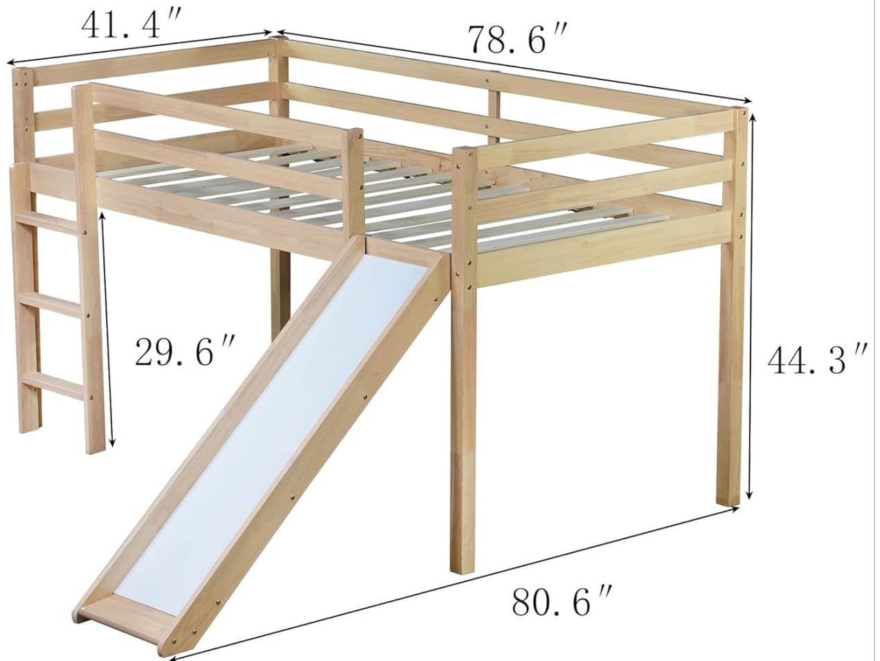
Image 7: Dimensional diagram of the loft bed.
