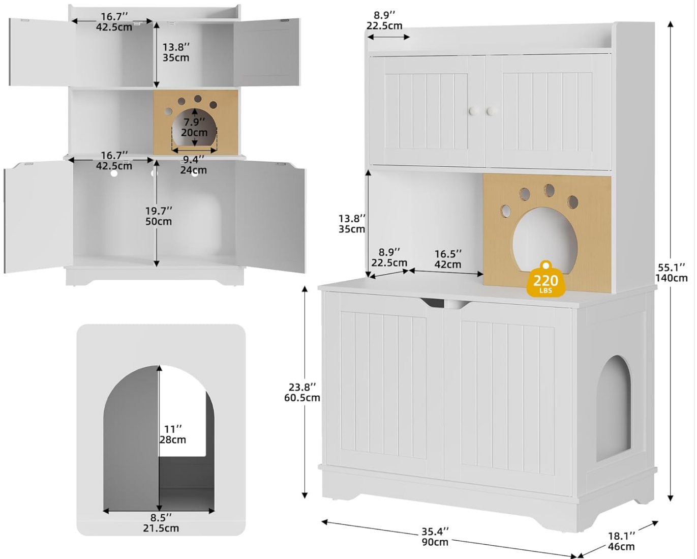
Figure 4.1: Diagram illustrating the dimensions and internal structure, useful for assembly.
