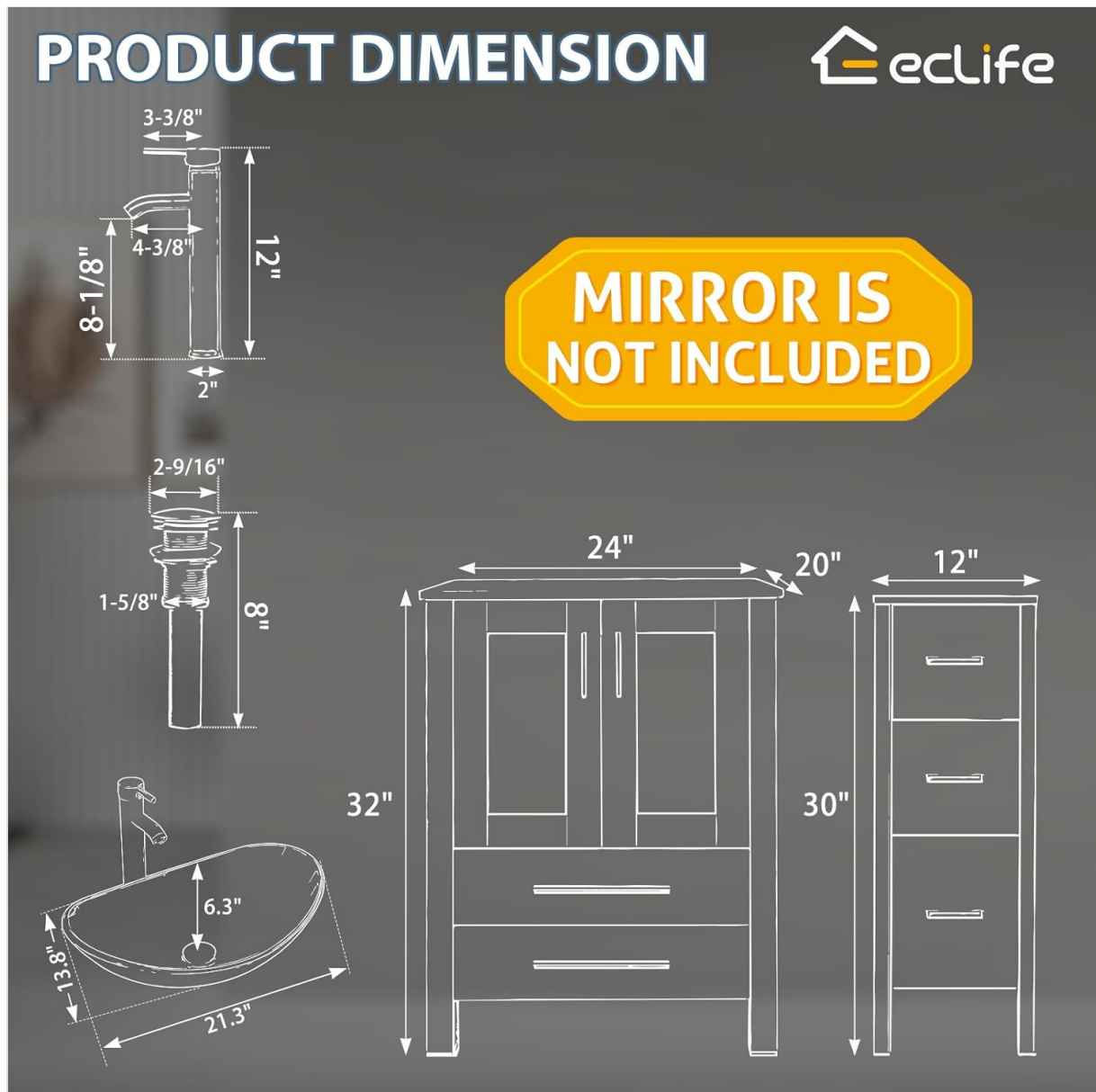
Image: Detailed product dimensions for the vanity, sink, and faucet.
