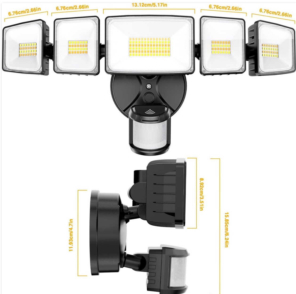
Image 3.2: Detailed dimensions of the Onforu 5-Head Smart LED Security Light, showing length, width, and height measurements.
