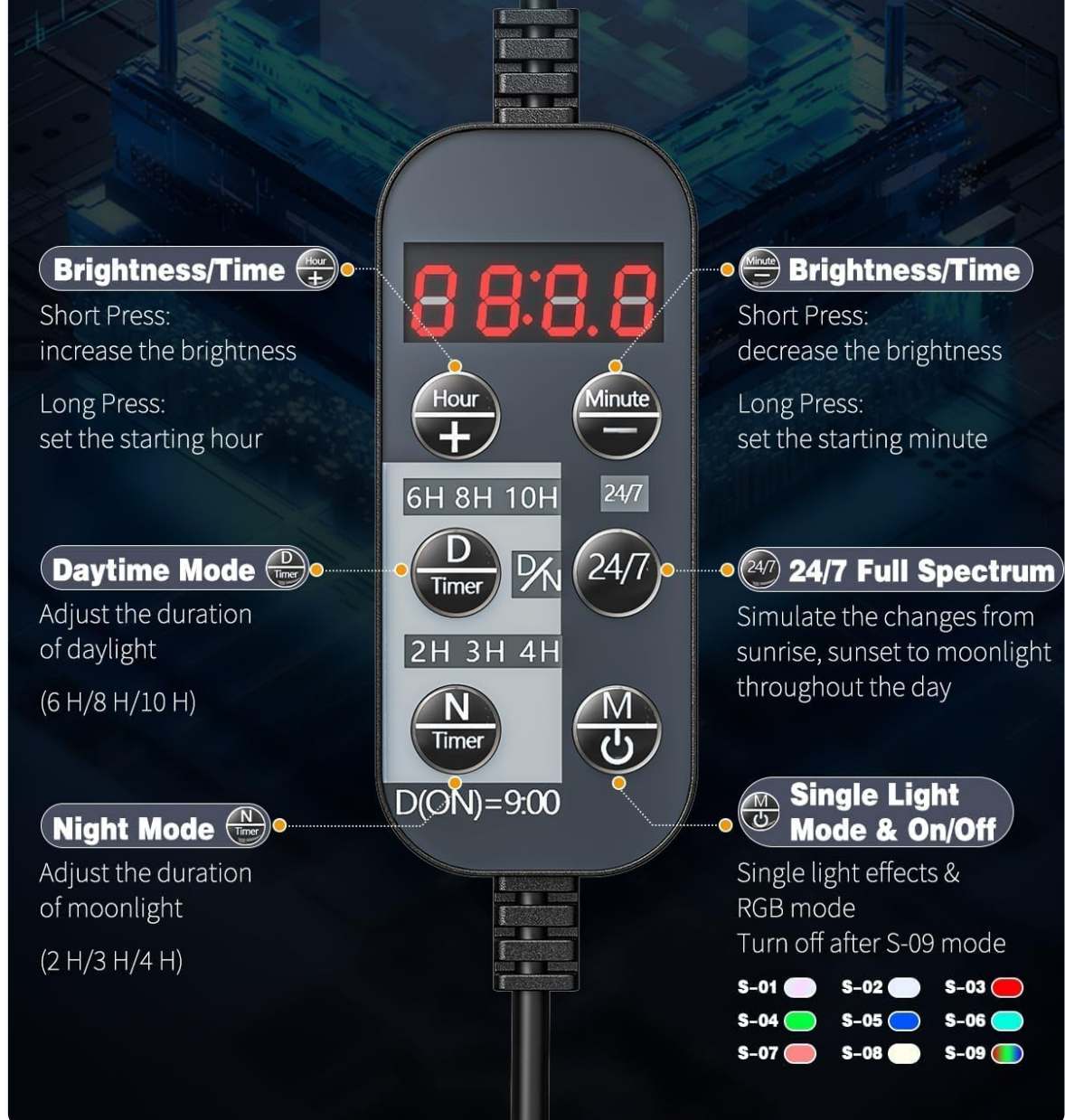
Image: Detailed view of the controller with buttons for Brightness/Time (increase/decrease, set hour/minute), Daytime Mode (6H, 8H, 10H), Night Mode (2H, 3H, 4H), 24/7 Full Spectrum, and Single Light Mode & On/Off (S-01 to S-09, OFF).
