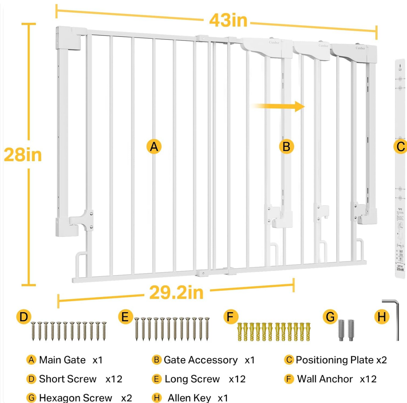
Figure 4.1: All components included in the package.
