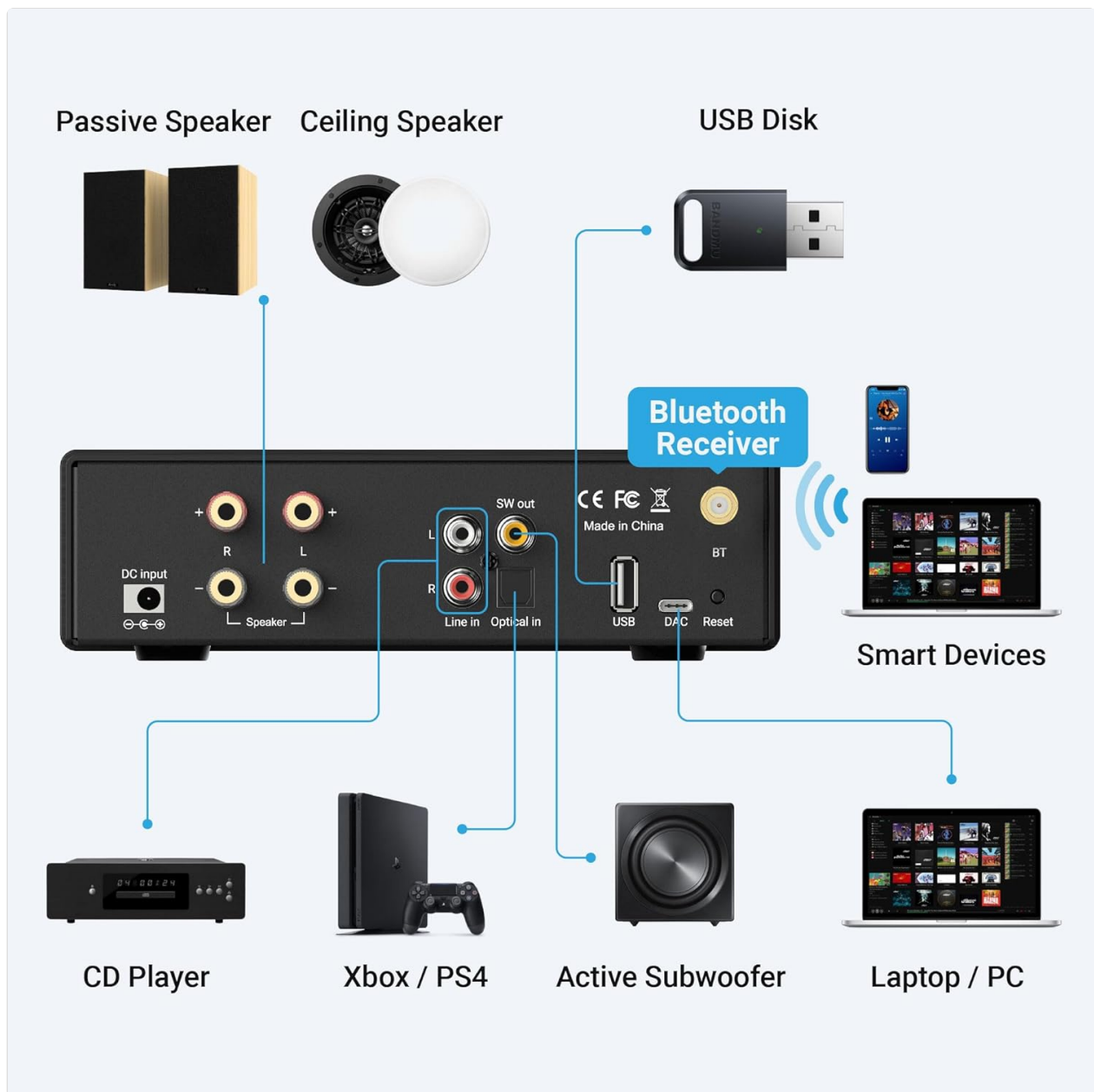
Figure 4.1: Rear panel connections of the Arylic B50SE.
