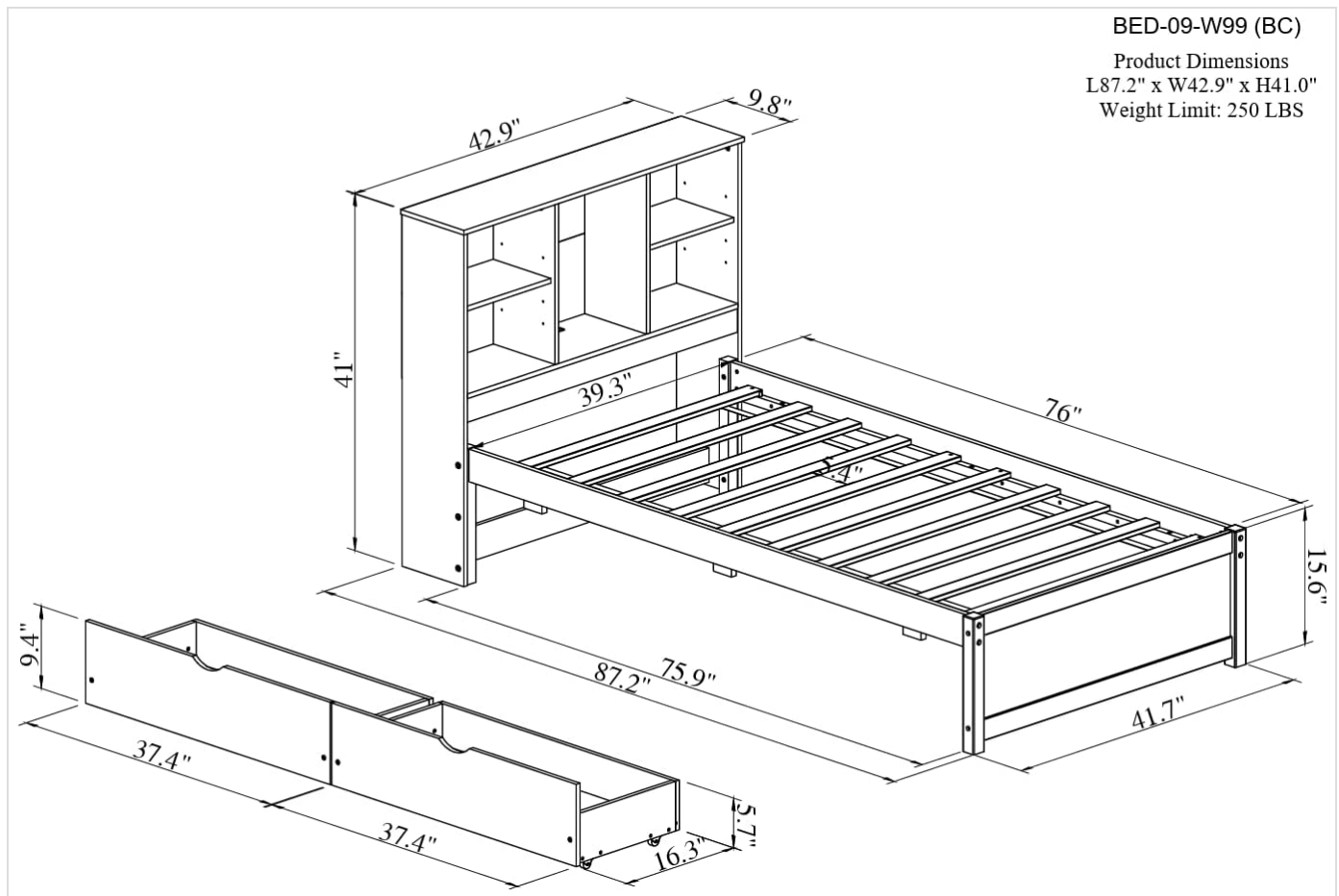
Figure 2: Front view of the assembled bed frame, showcasing the headboard storage and under-bed drawers.
