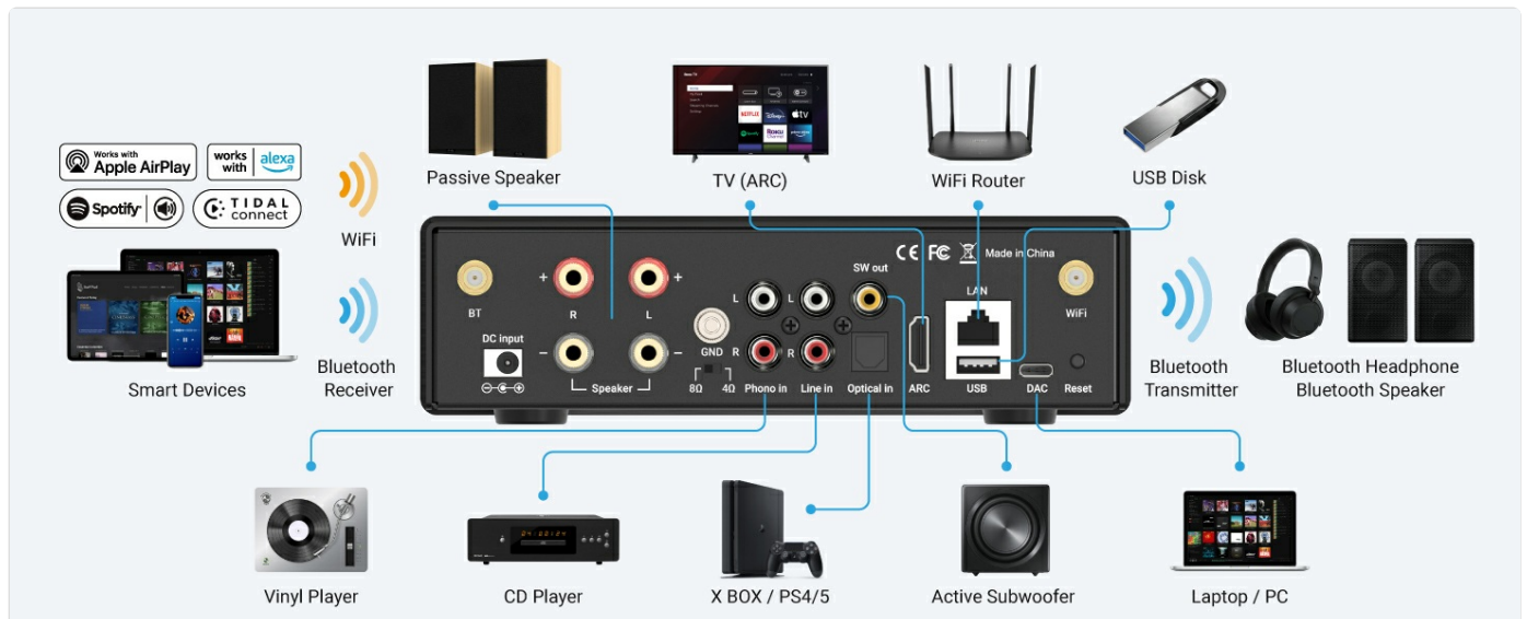
Figure 9: Comprehensive connection diagram for the Arylic H50.
