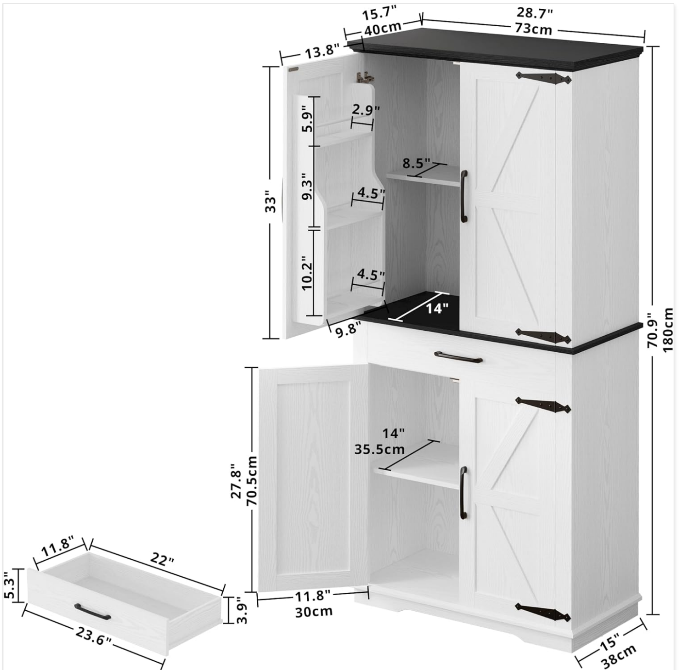
Image: Diagram illustrating the dimensions and various components of the pantry cabinet, including the upper and lower sections, drawer, and door shelves.
