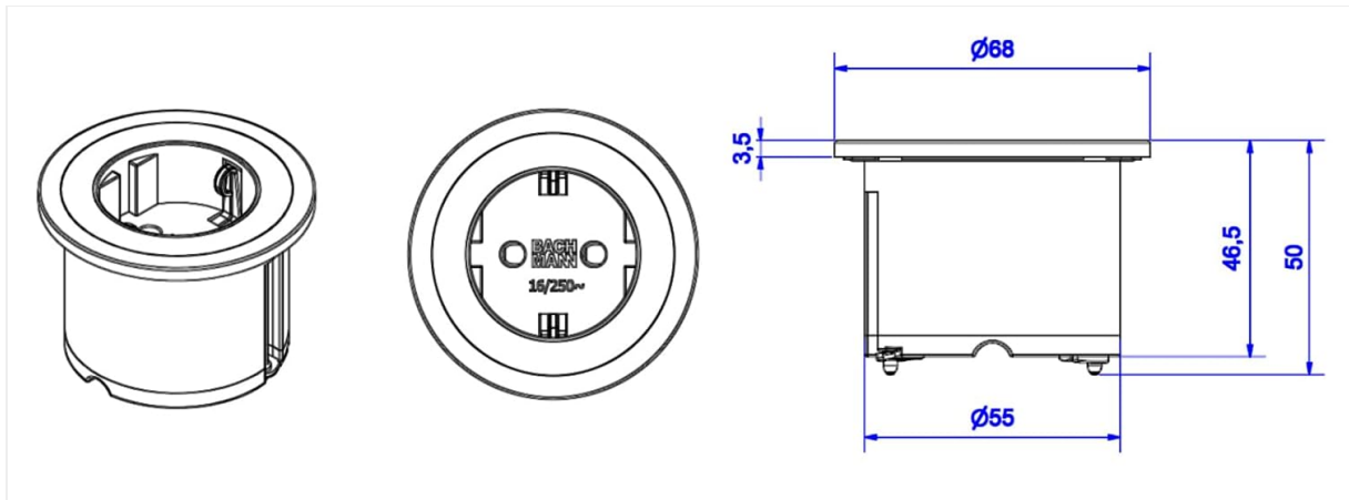
Figure 5.1: Dimensional drawing for installation planning.
