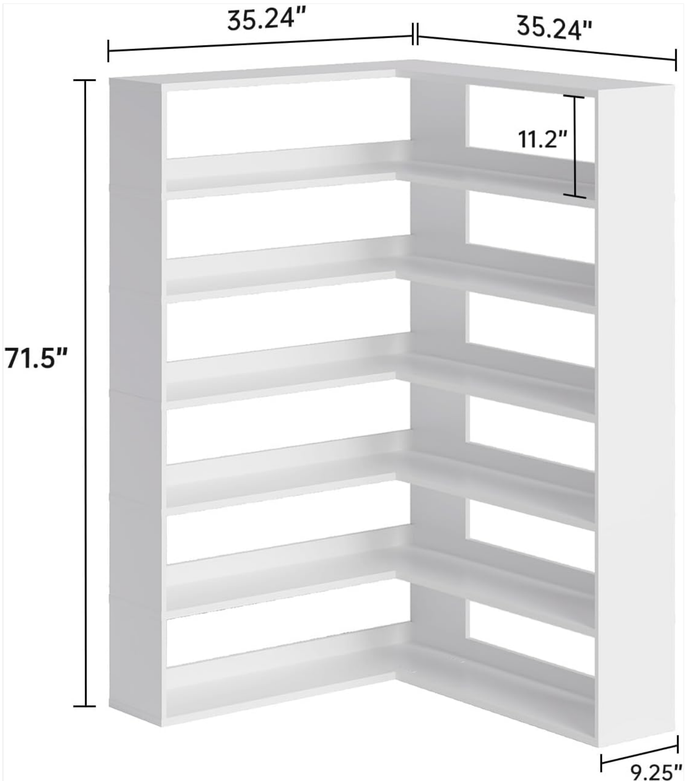
Figure 3.1: Bookshelf Dimensions. The unit measures 71.5 inches in height, with each L-shaped side extending 35.24 inches in width and a depth of 9.25 inches.
