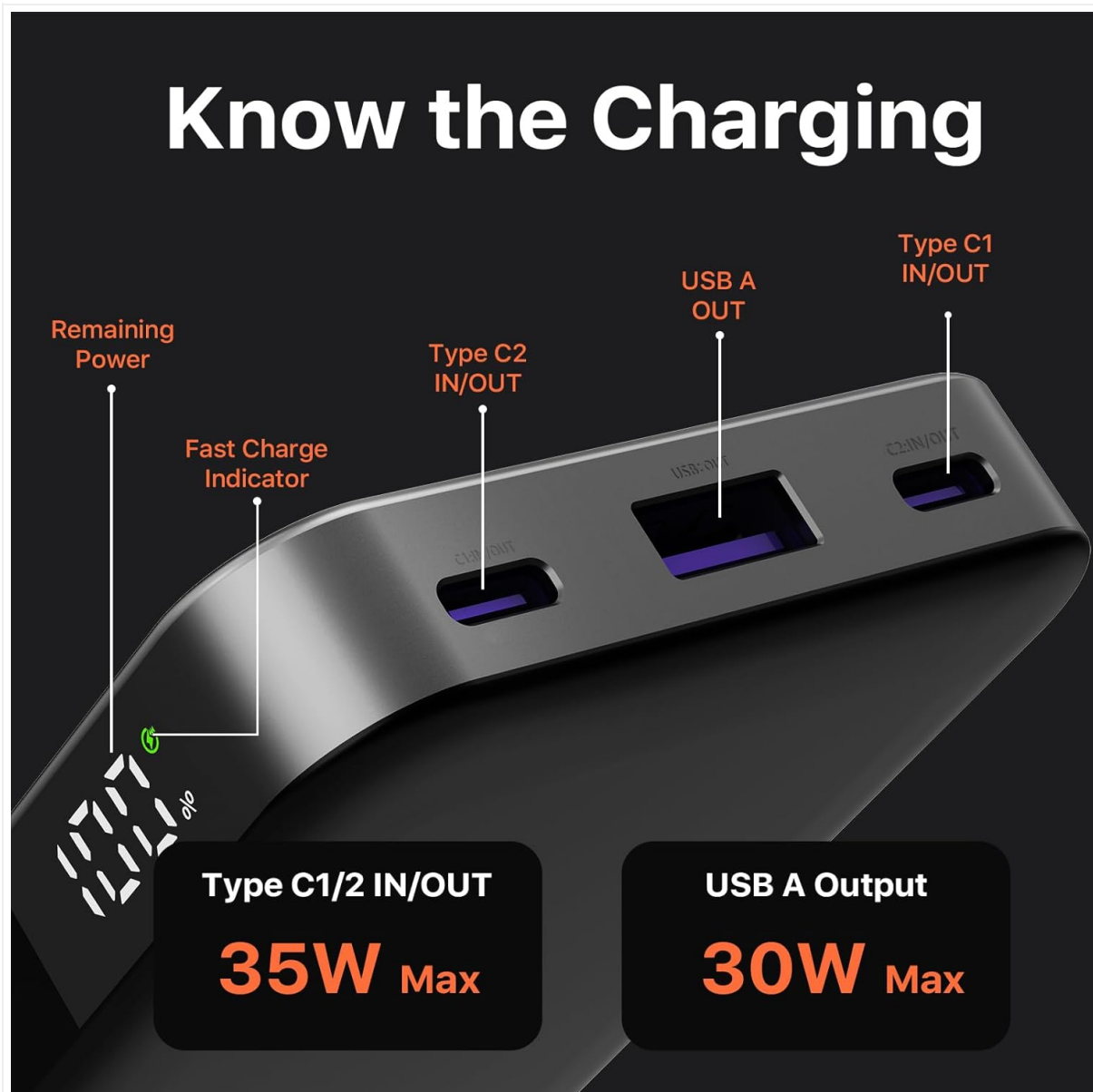
Image: Detailed view of the 35W power bank's interface, highlighting the digital display and port functions.
