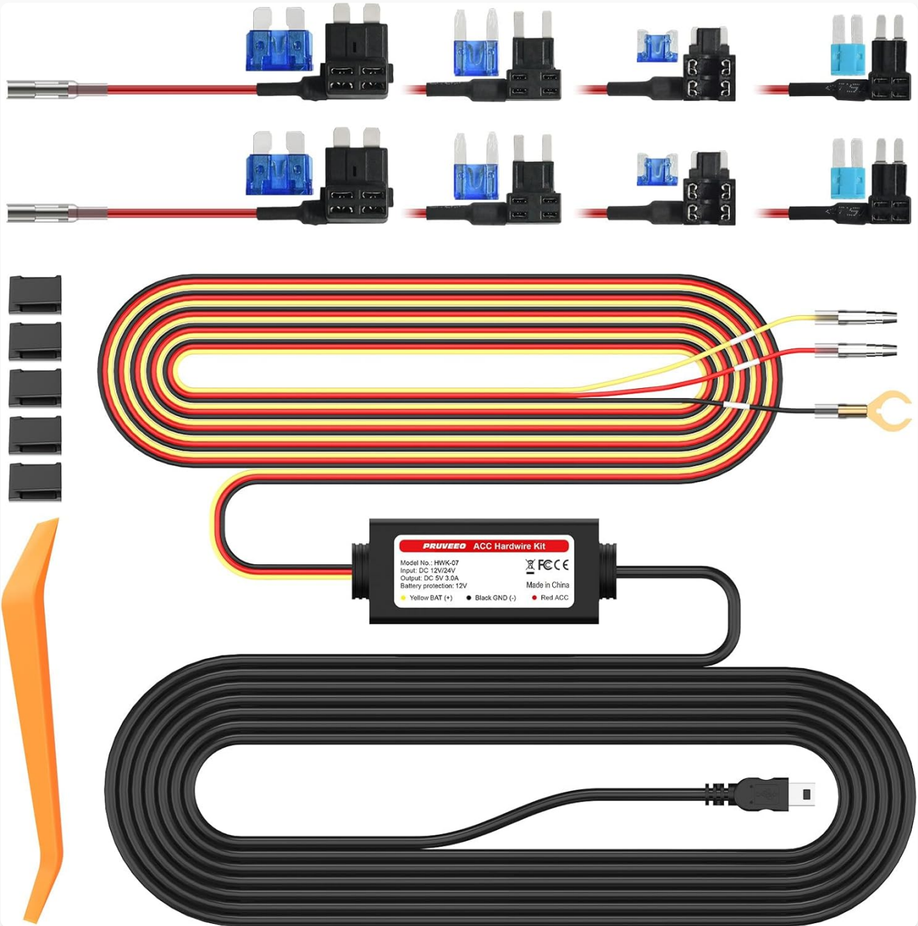
Image 3.1: Components of the ACC Hardwire Kit.
