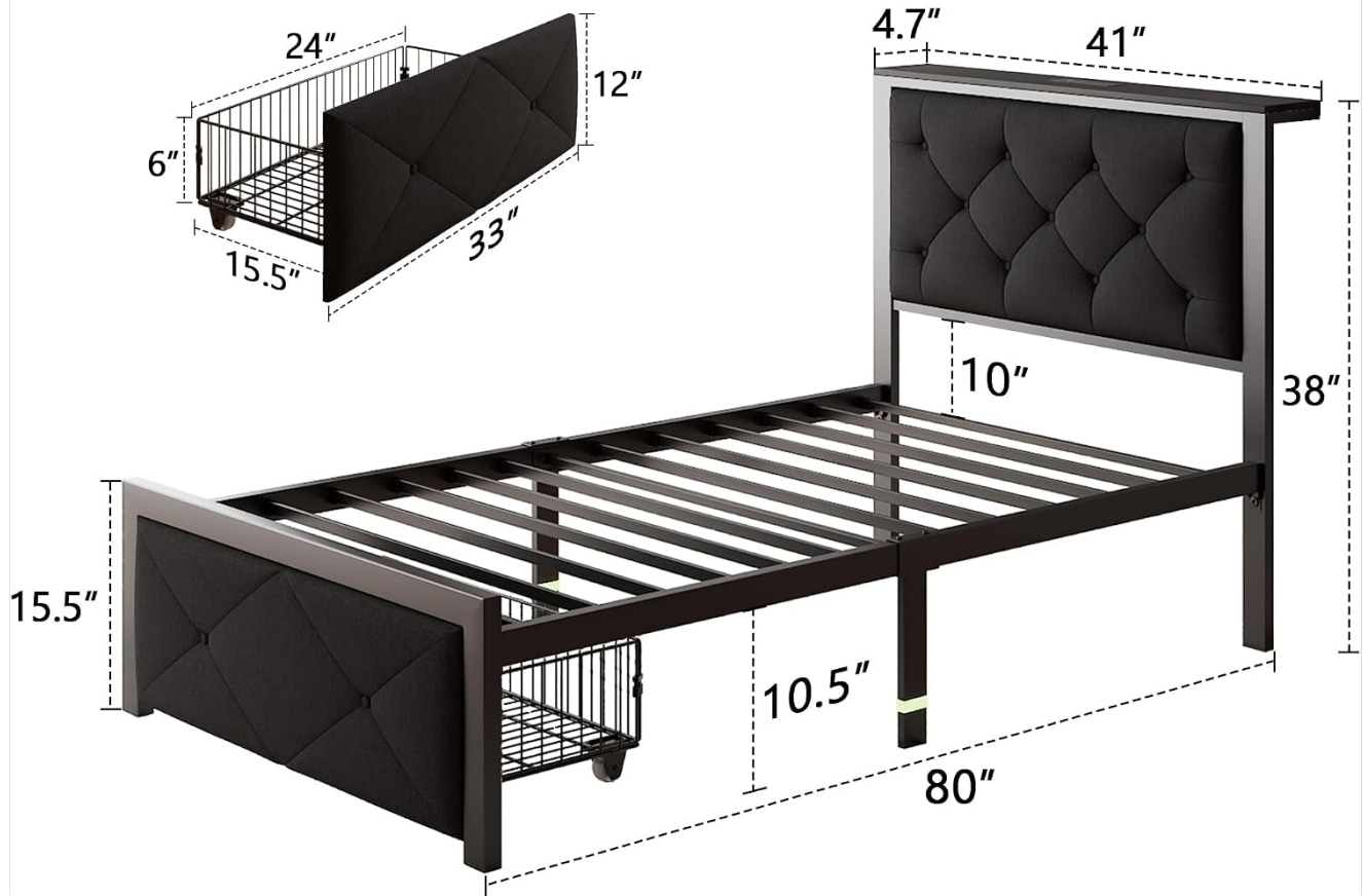
Image 8.1: Key dimensions and features of the Feonase Twin Platform Bed Frame.
