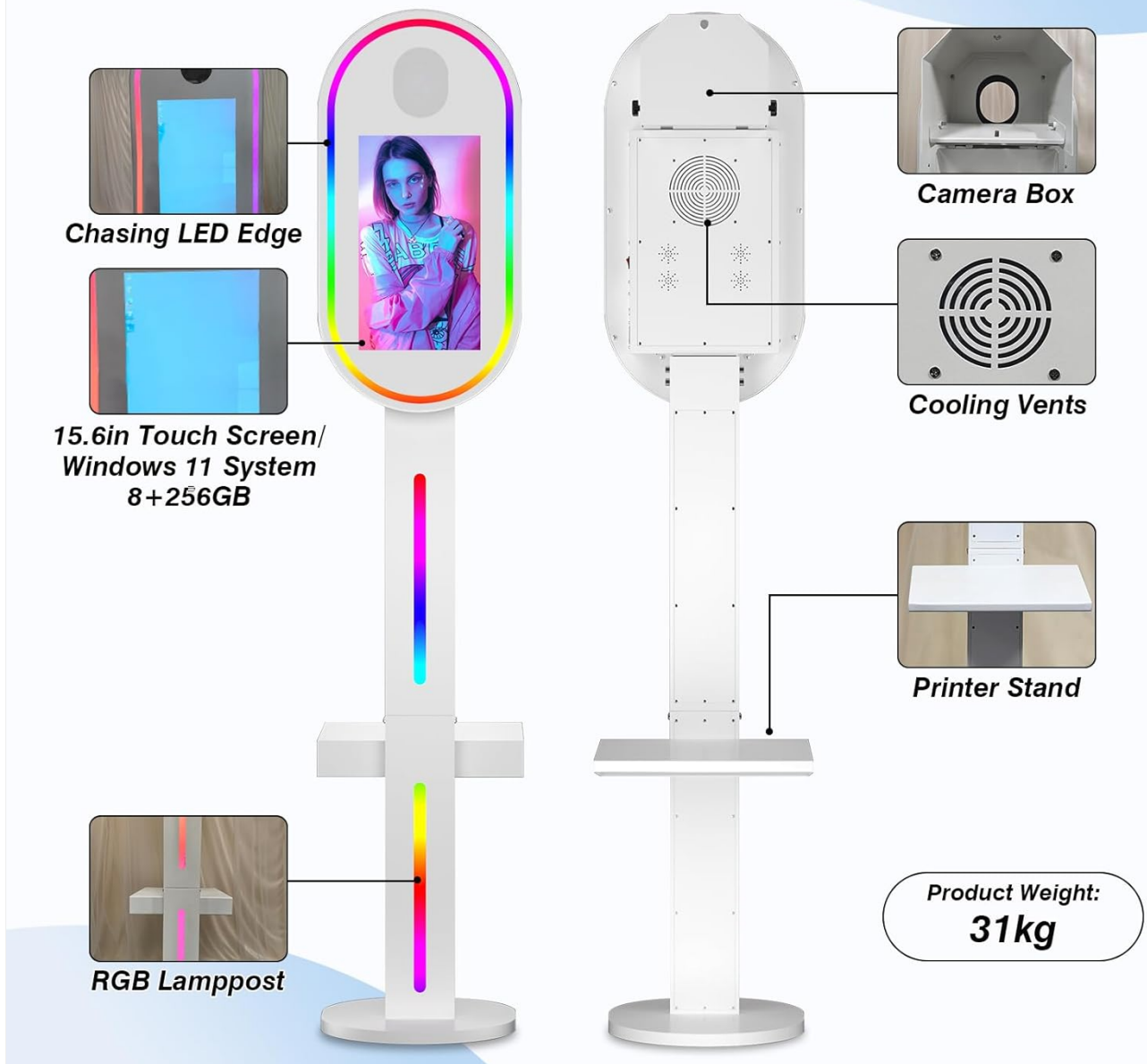
Figure 3: Detailed view of the photo booth's internal components and external features, including the camera box, cooling vents, and RGB lamppost.
