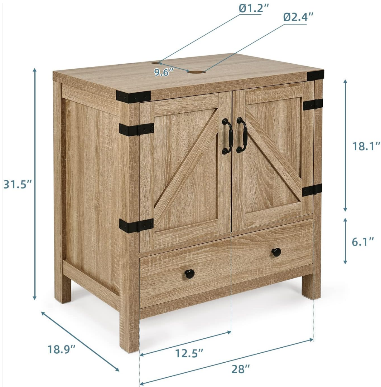
Image: Detailed dimensions of the vanity cabinet.
