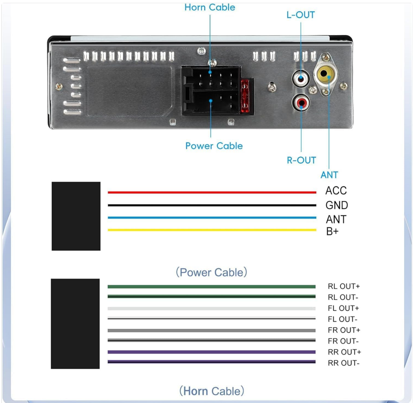
Figure 4.1: Detailed wiring diagram for the CAMECHO car stereo, showing connections for ACC, GND, ANT, B+, and speaker outputs (RL, FL, FR, RR).
