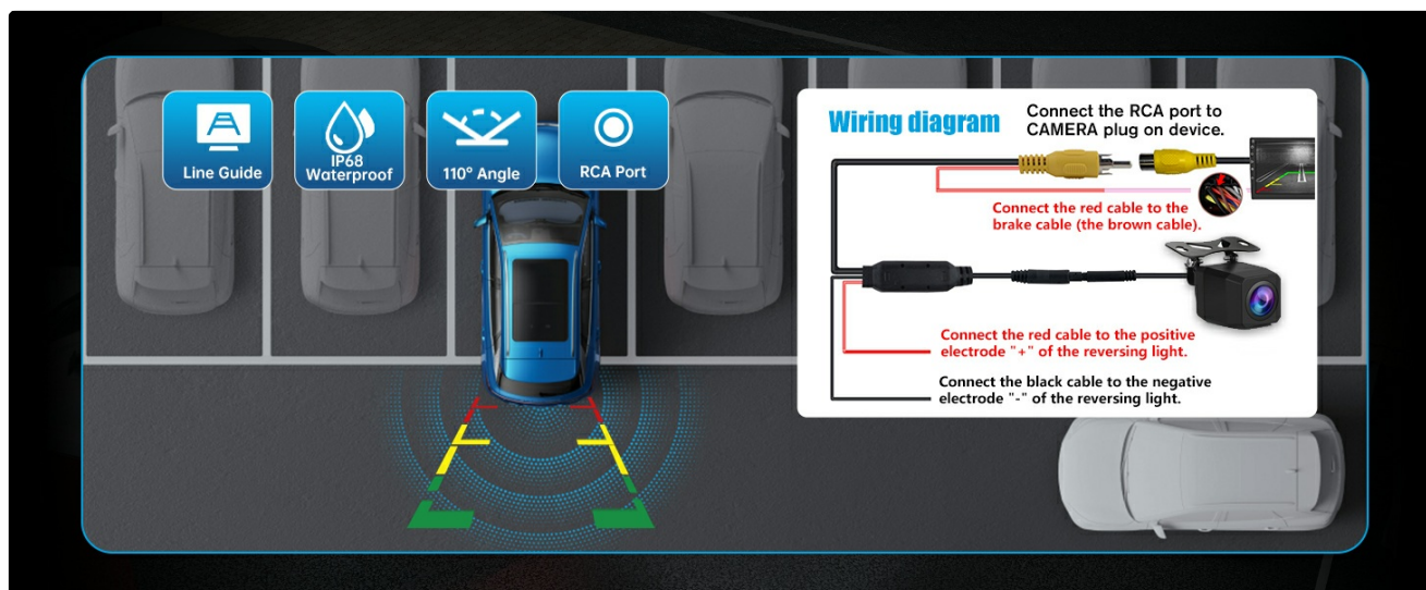
Figure 4.2: Backup Camera Wiring Diagram
