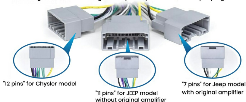
Figure 4.3: Wiring Harness Plug Selection
