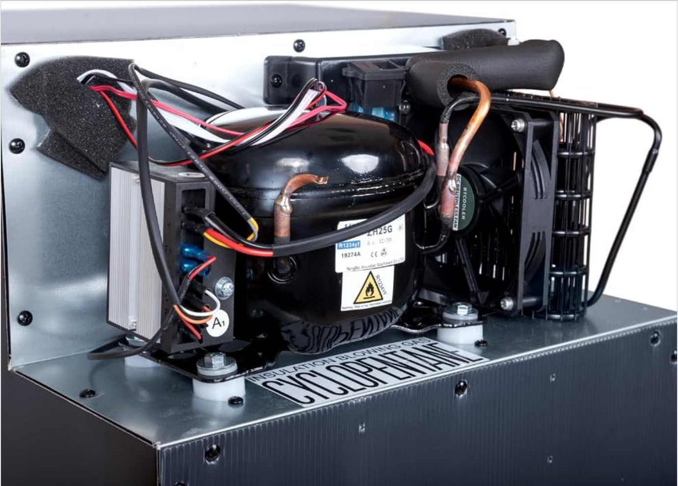
Image 8.1: Close-up view of the compressor unit.
