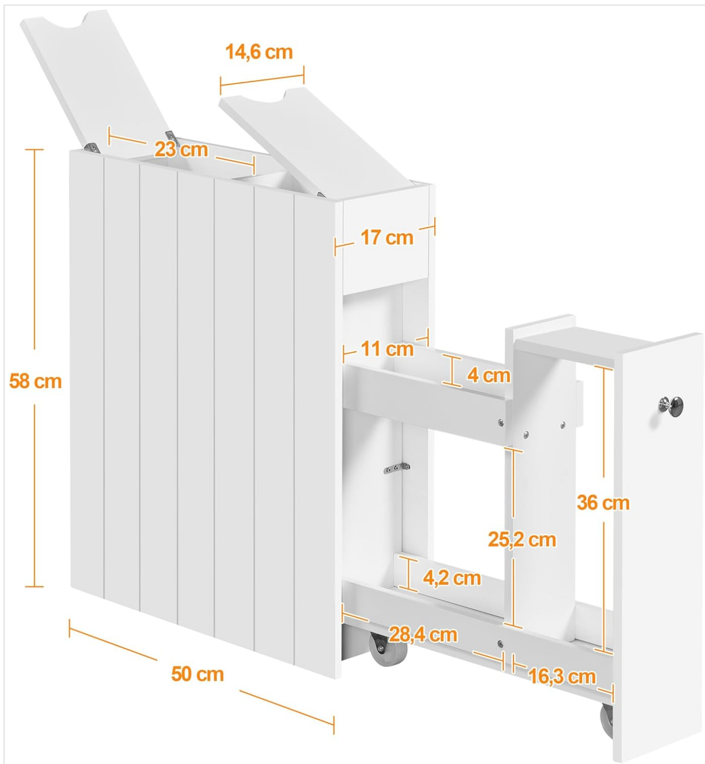
Figure 1: Product Dimensions. This image illustrates the overall dimensions of the cabinet, including length, width, and height, along with internal compartment measurements.
