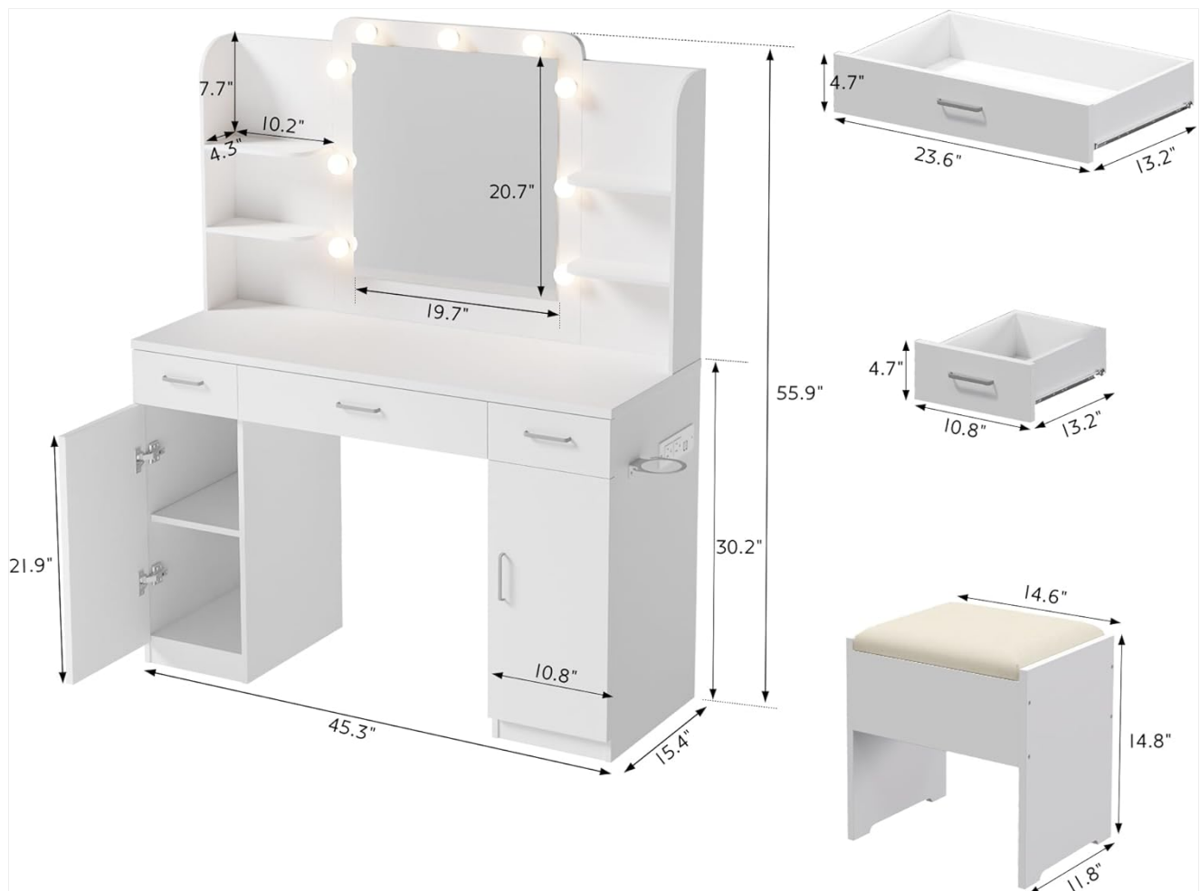
Figure 2: Vanity Desk and Stool Dimensions.
